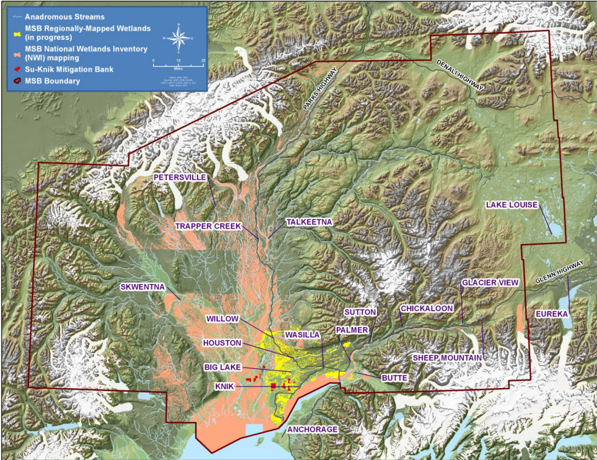
Figure 6: MSB Regionally Mapped and NWI Mapped Wetlands
