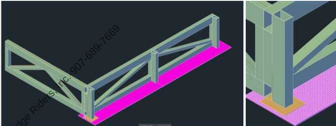
Figure 9 - Foundation Design
