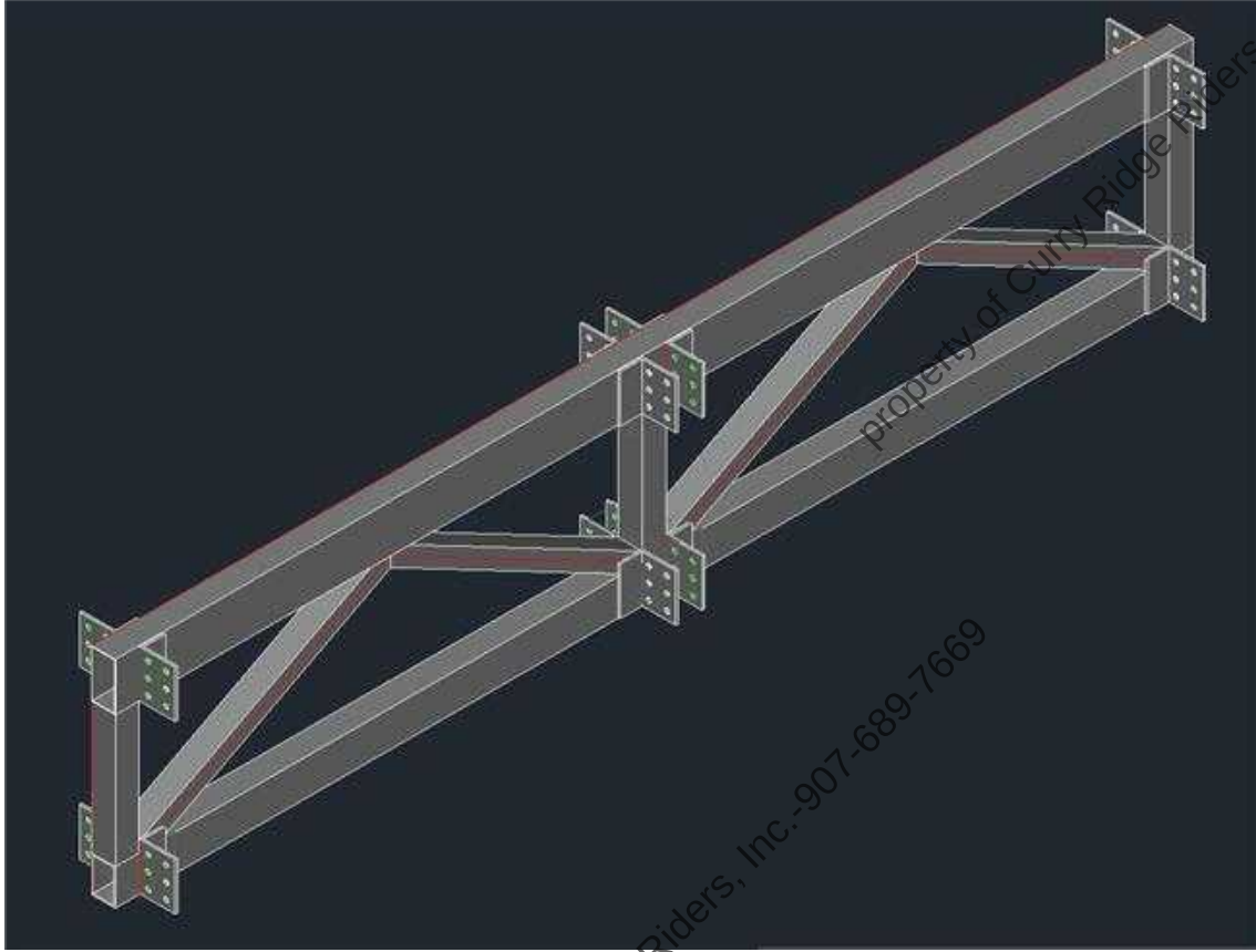
Figure 6 - Lateral Frame Rendering
